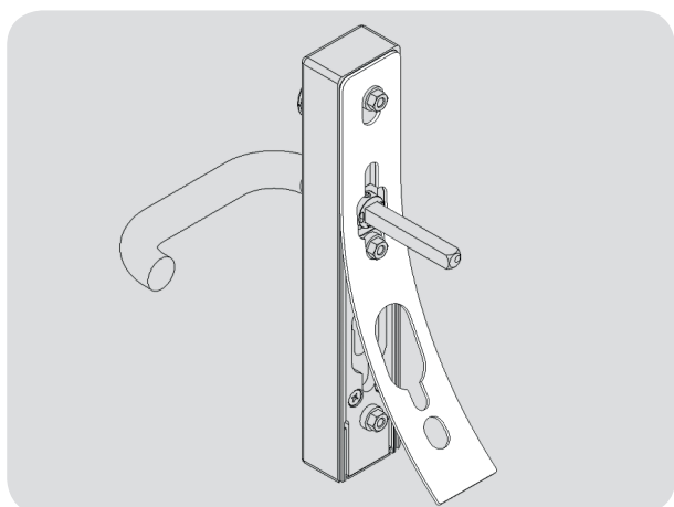
Fig. 13: Applying the sealing mat
